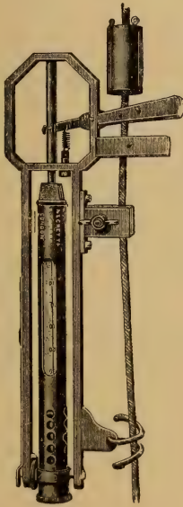
FIG. 8.—FRAME OF REVERSING THERMOMETER.
